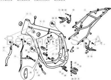
TAV.31 Telaio - Frame - Chassis - Rahmen - Chasis
