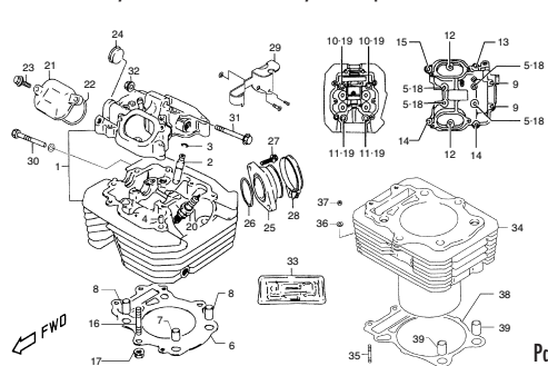
TAV.2 Testa-cilindro - Cylinder head - Culasse - Zylinderkopf - Culata
