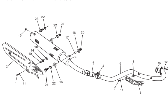
TAV.10 - Marmitta - Silencers
