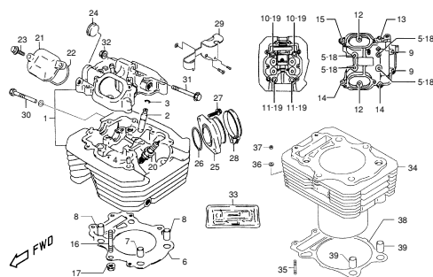
TAV.2 - Testa-cilindro - Cylinder head
