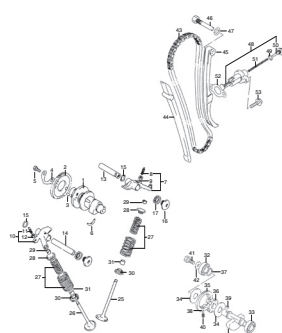
TAV.5 - Albero a camme-valvole - Camshaft-Valves
